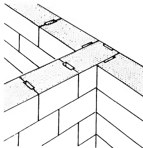
8 Poroton blocks with mortar filling
